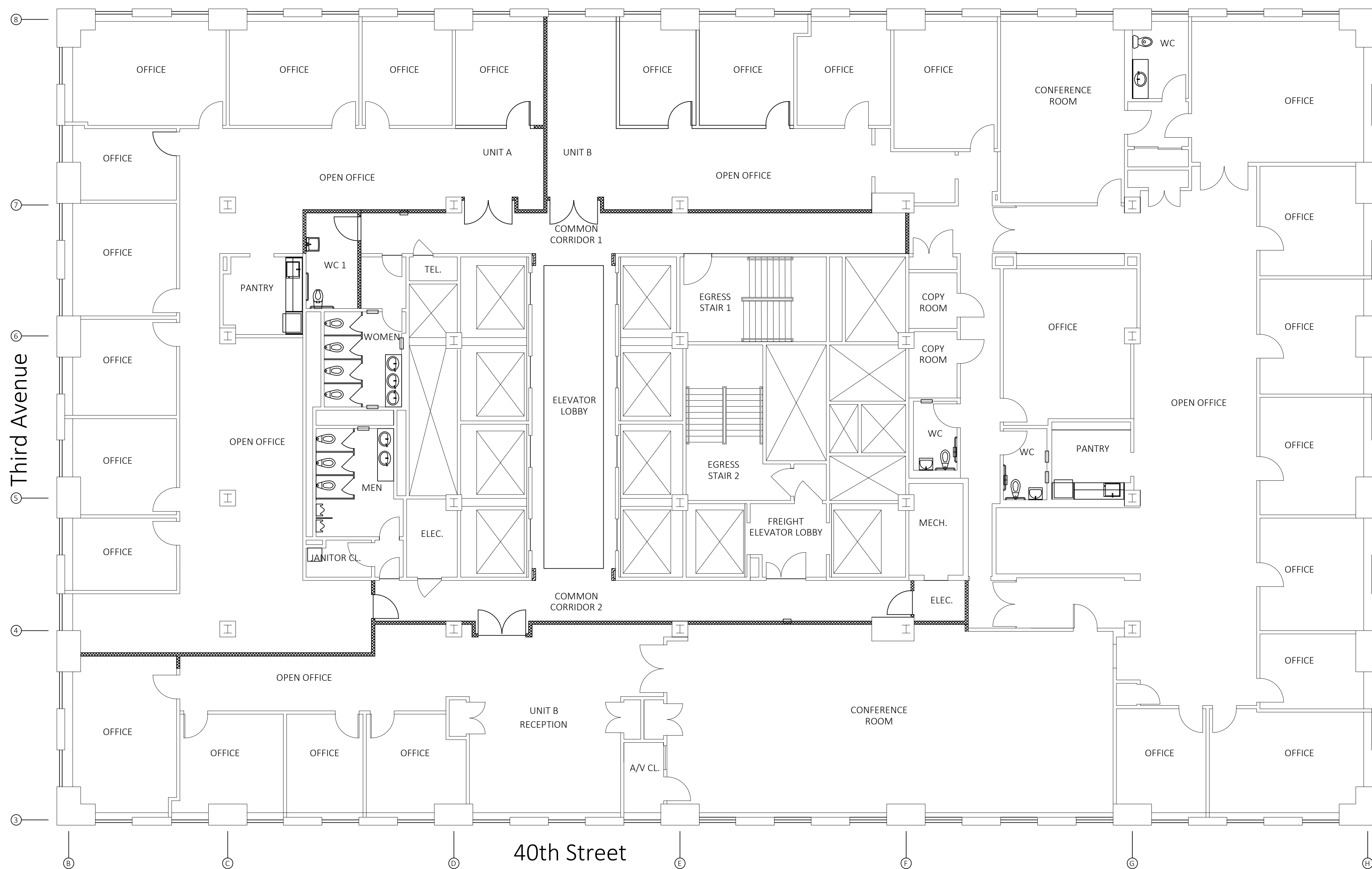
1 PROPOSED PLAN : FLOOR 38 1/8"=1'-0"
